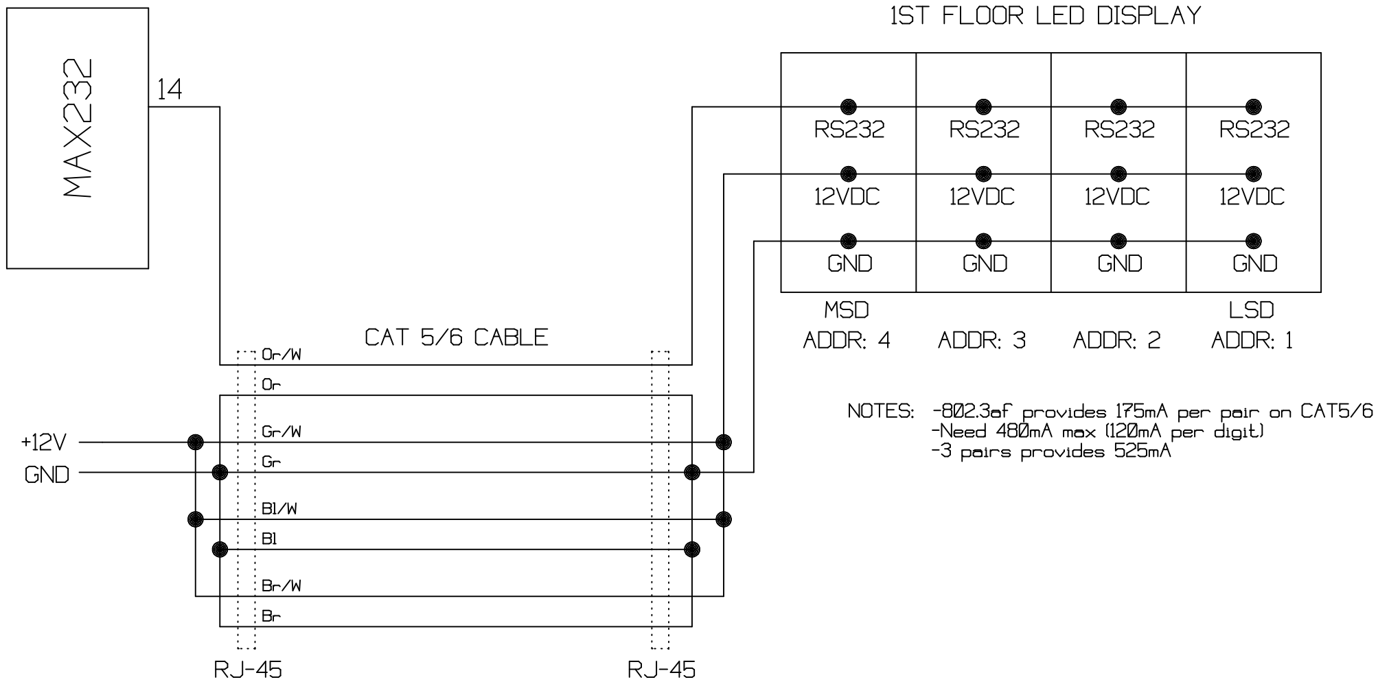
DETAIL 4 - WIRING TO 1ST FLOOR LED DISPLAY
